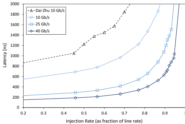
Figure 20: Latency vs. injection rate of the NoC-based Ethernet switch given line rates of 10, 25, and 40 Gb/s, and compared to the Dai/Zhu 16×16 10 Gb/s FPGA switch fabric design [11]. Our switch queues and Dai/Zhu’s switch queues are of size 60kb and 16kb, respectively.
